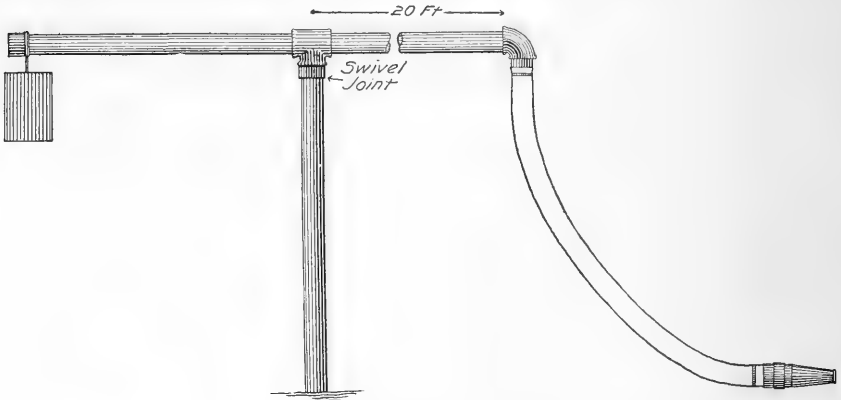
FIG. 4.—Adjustable hydrant with hose and nozzle.
